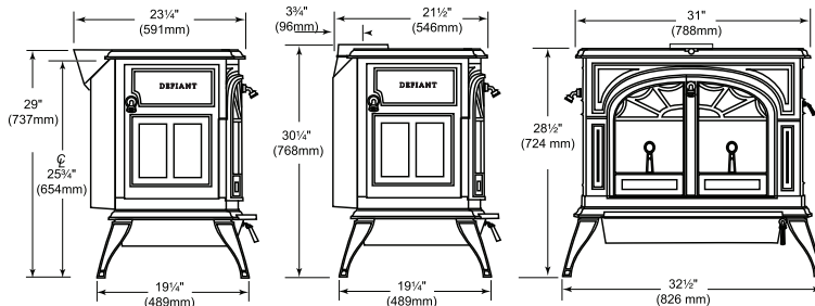
Flue collar in Rear Vent position
